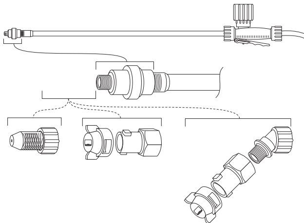
Female (3) and male (4) adapters with diaphragm
